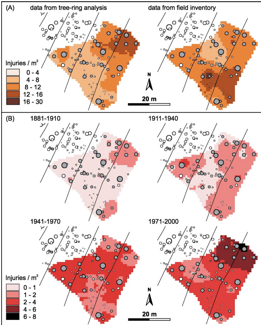
Fig. 5. Reconstructed spatial rockfall distribution in the investigated perimeter (see Fig. 1). Maps show the interpolated (linear, with 10 neighbouring trees) number of injuries per \text{m}^2 . (A) Data from tree-ring analysis versus data from field inventory. (B) Data from tree-ring analysis divided into four time sequences covering 30 years each.
