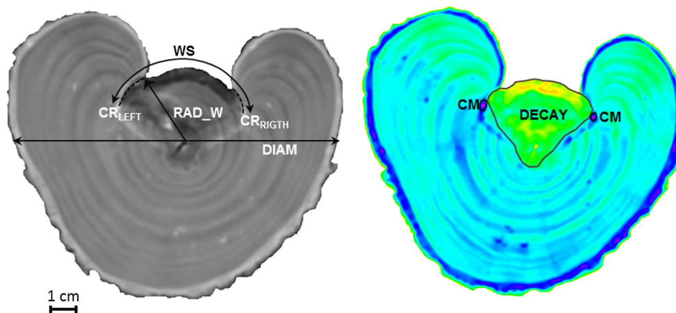
Fig. 1 Definition of parameters measured on XRCT slices: ( left ) DIAM represents the diameter of the tree measured perpendicular to the damage, RAD_W indicates the radius at the moment of impact, WS represents the length of damaged cambial tissue, and CR LEFT and CR RIGHT are the lengths of the callus; ( right ) DECAY represents the
