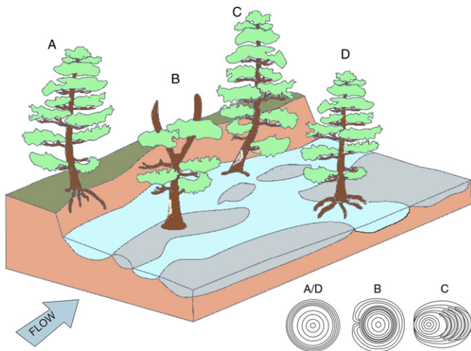
Fig. 3. Predominant dendrogeomorphic macro-evidence in trees affected by flash floods and associated responses in tree-ring width and cell structure: (A/D) root exposure; (B) sheared off tree and candelabra growth; (C) stem tilting; (B/C) injuries.
