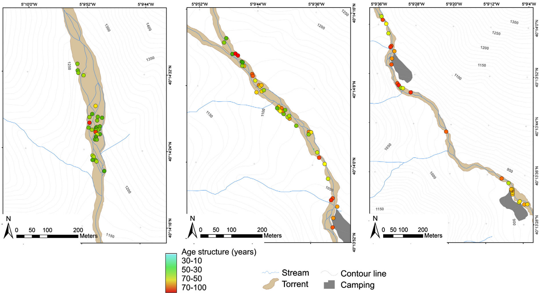
Fig. 7. Age structure of the sampled trees in the torrent. Left: upper sector of the study reach. Right: lower sector.
