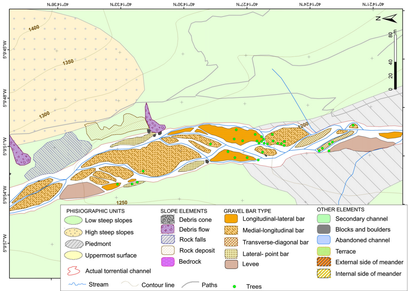
Fig. 5. Geomorphological mapping of the upper part of the study reach. The legend shows the classification of units and elements.
