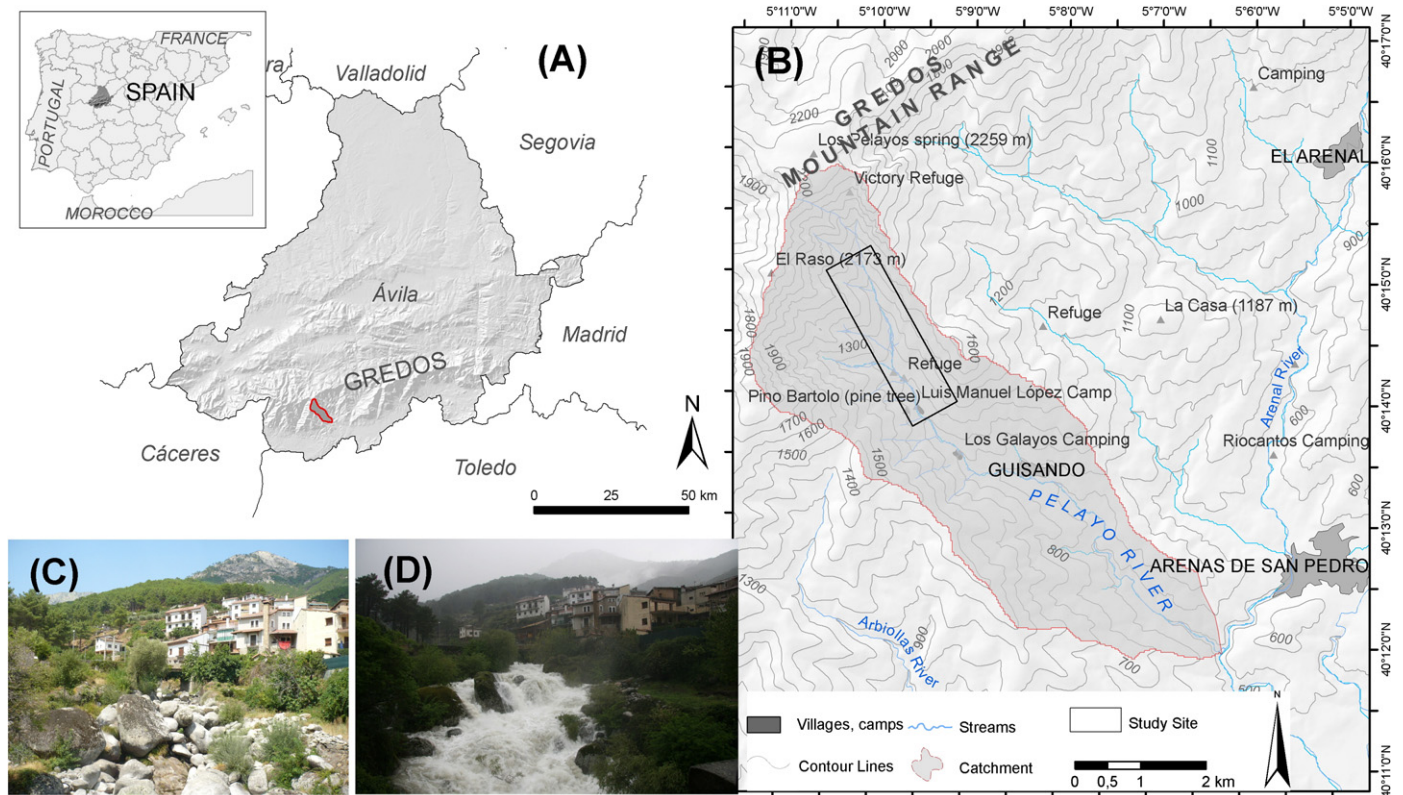
Fig. 1. (A) Location of the study area in the Gredos Mountain Range (Spanish Central System); (B) overview of the Pelayo River catchment and the study site of this analysis; (C) the Pelayo River at Guisando village during normal conditions and (D) during the flash flood event in December 2008 (picture of 2008 flash flood event, courtesy of Gloria Suarez García, used with permission).
