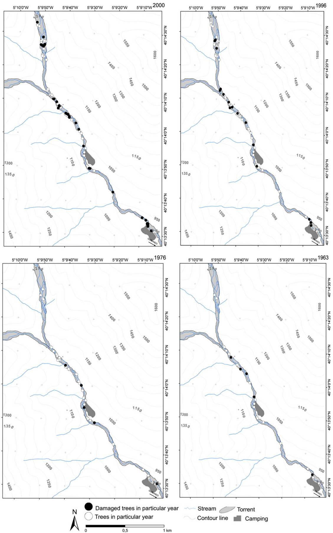
Fig. 8. Spatial distribution of living and damaged trees of four dated events.
