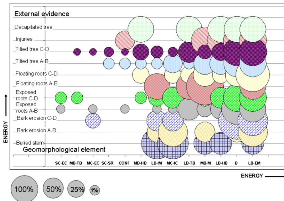
Fig. 6. Relation between the energy of the external evidence and the geomorphological elements. Ball size represents the percentage of trees showing a specific disturbance located in a specific geomorphological side related to the total number of trees showing that disturbance. The legend may be checked in Table 5.
