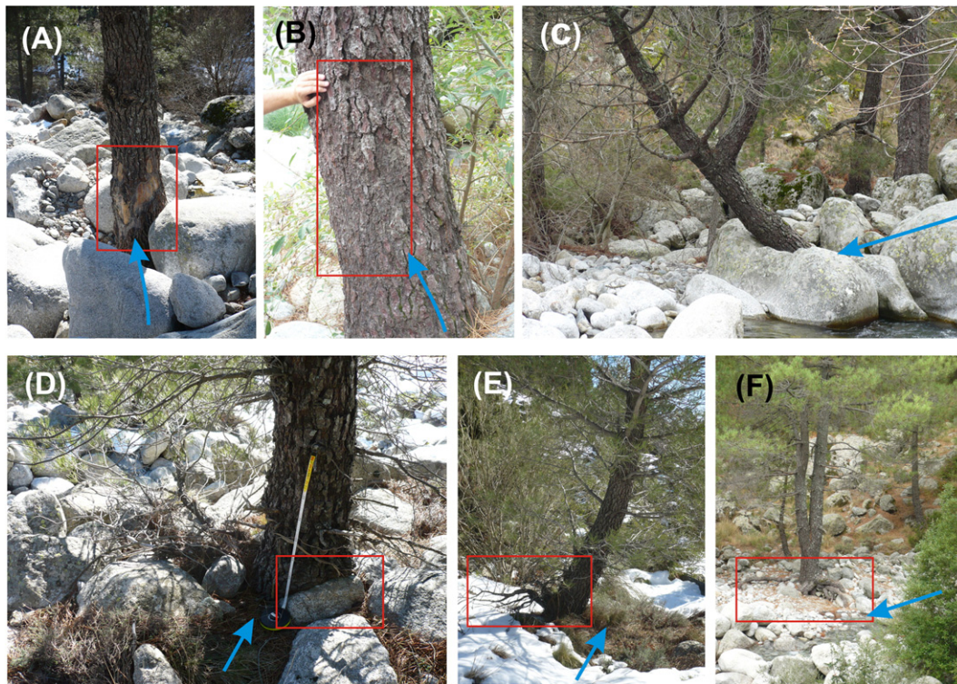
Fig. 4. External evidence of flash flood activity in trees growing along the Pelayo River: (A) abrasion scars; (B) bark erosion; (C) stem tilting; (D) stem burial; (E) floating roots; (F) exposed roots. The blue arrows indicate the flow direction.
