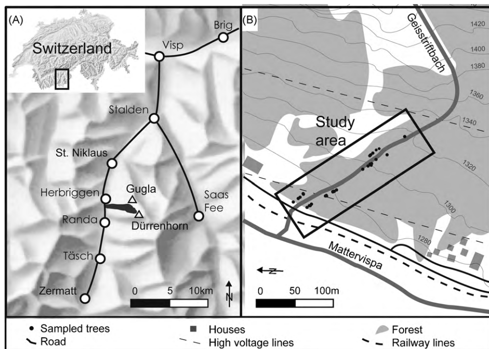
Fig. 1. (A) The catchment area of the Geisstriftbach torrent is located in the southern Swiss Alps (Valais) between the settlements of Herbruggen and Randa. (B) Sketch map of the study area and position of trees sampled along the channel of the Geisstriftbach.
